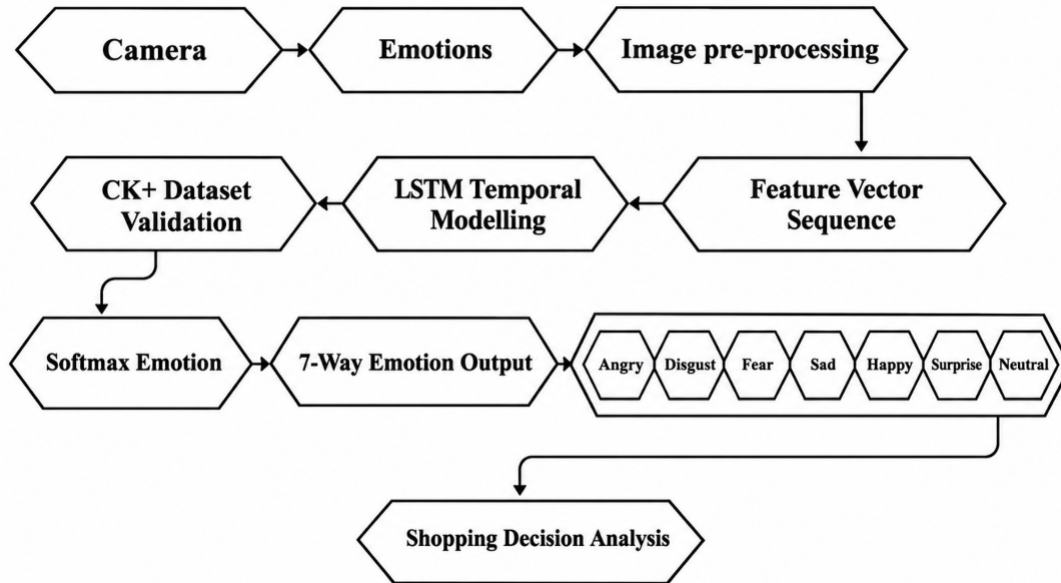
Figure 1: LSTM pipeline: CCTV input → face detection → preprocessing → LSTM temporal modelling (validated on CK+) → Softmax 7-class emotion classification → shopping decision analysis.
