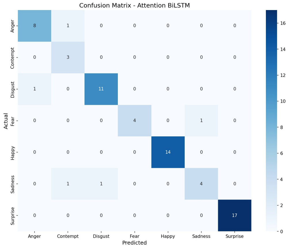
Figure 2: Attention BiLSTM confusion matrix on CK+. Happy and surprise achieved 100% recall. Primary confusion occurred between anger and contempt.
