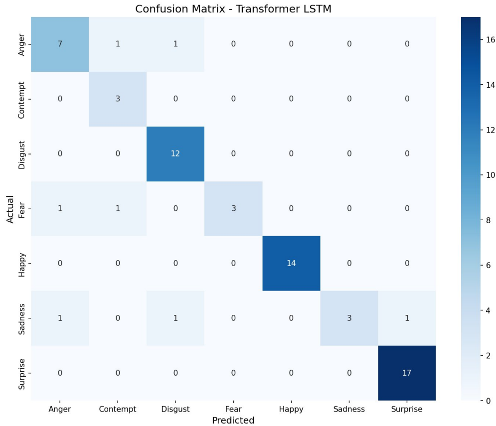
Figure 5: Transformer–LSTM confusion matrix. Perfect classification of disgust, happy, contempt, and surprise. Errors concentrated in anger–fear discrimination.
