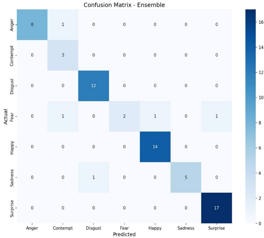
Figure 8: Ensemble confusion matrix combining all four LSTM models. Accuracy (92.42%) did not exceed the best individual model, indicating that error patterns across architectures were subsets rather than complements.
