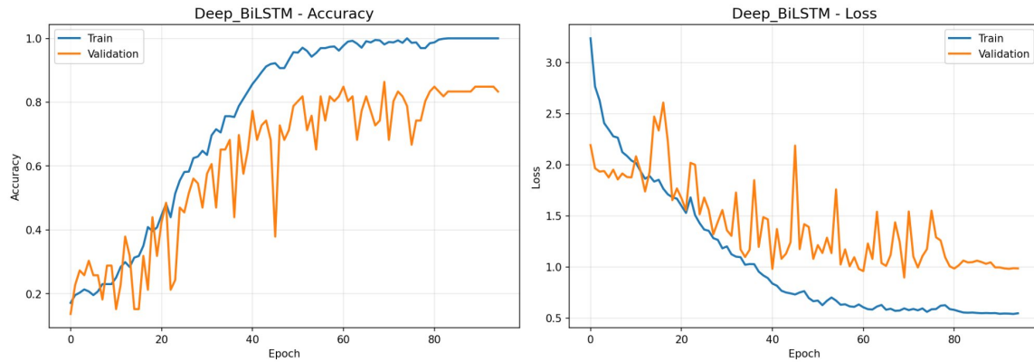
Figure 6: Deep BiLSTM training curves on CK+. Extended training (95 epochs) did not achieve accuracy comparable to the simpler Attention BiLSTM, suggesting that additional depth was counterproductive.
