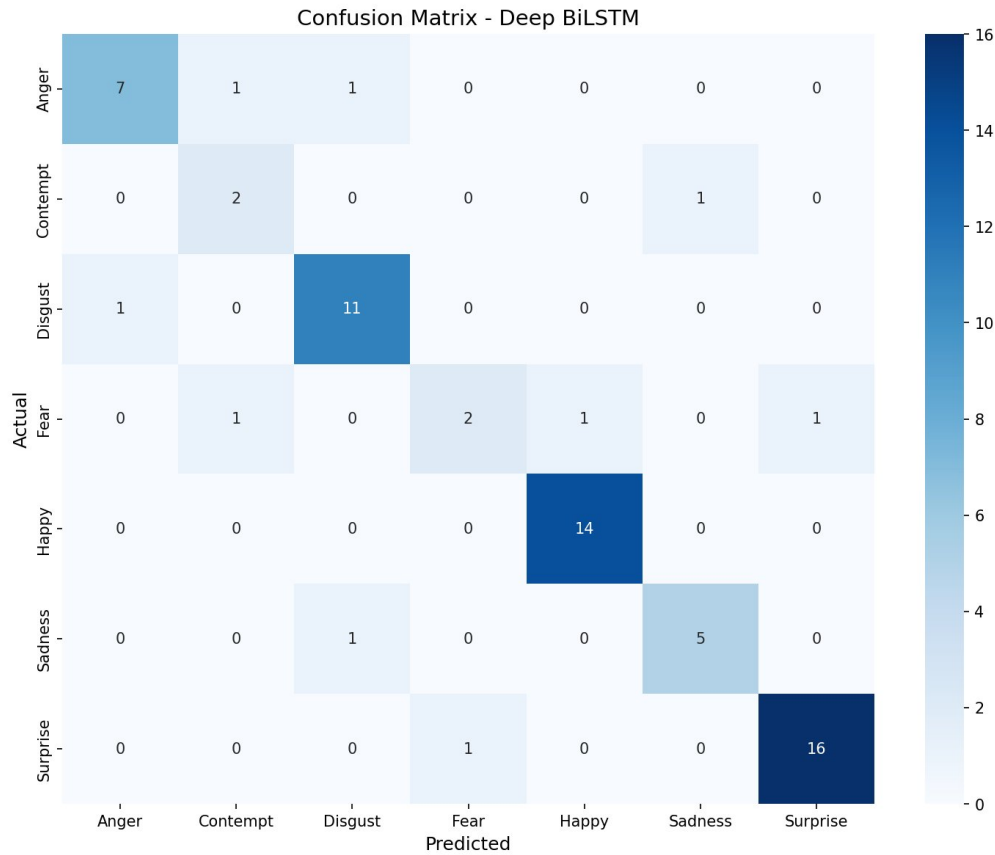
Figure 7: Deep BiLSTM confusion matrix (86.36% accuracy). Despite having the most parameters among individual models, performance was below Attention BiLSTM across most emotion categories.
