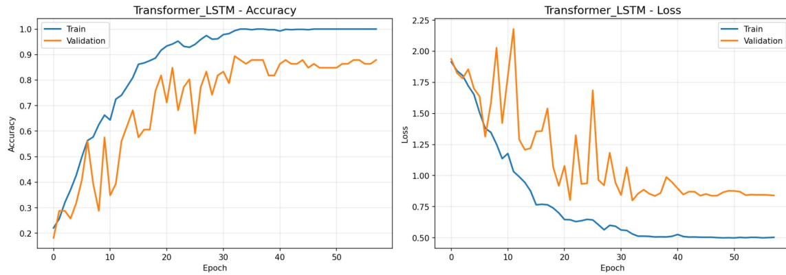
Figure 4: Transformer–LSTM training curves on CK+. Validation accuracy reached 89% with multi-head self-attention. Slower convergence than Attention BiLSTM.
